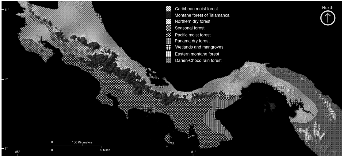
FIGURE 7. Vegetation units of Costa Rica and Panama.
