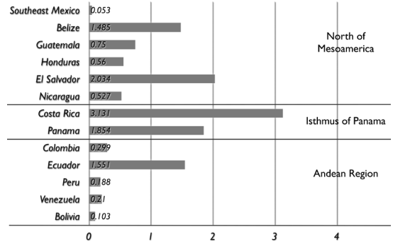
FIGURE 2. Comparison of the number of species between northern Mesoamerica, Isthmus of Panama, and the Andean countries.
